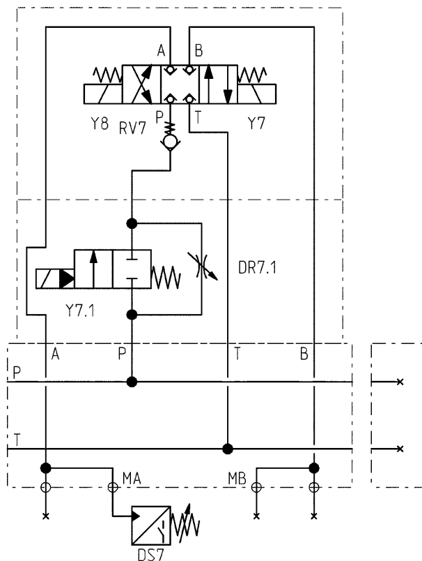
Spacer plate with connectable throttle Function in P
