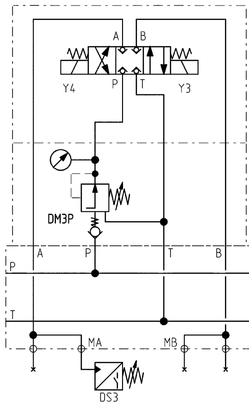
Spacer plates - 3-way pressure-control valve Control function in P
