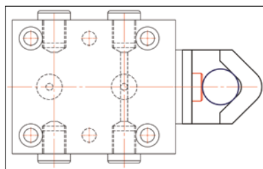
Clamping of workpiece with mouled lugs.
