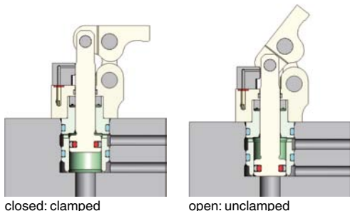
closed: clamped
